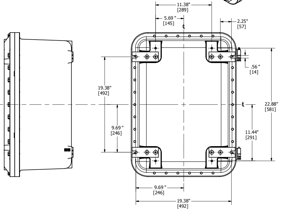
MOUNTING FEET
